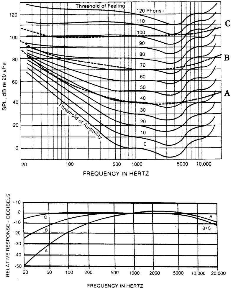
FIGURE 16.2 Top: Equal loudness contours based on the psychophysical phon scale, with sound level meter frequency weighting curves superimposed. Bottom: dB vs. frequency values of A, B, and C sound level meter weighting curves. (Adapted from Earshen, J. J. [1986]. Sound measurement: Instrumentation and noise descriptors, in E. H. Berger, W. D. Ward, J. C. Morrill, and L. H. Royster [Eds.], Noise and Hearing Conservation Manual [pp. 38-95]. Akron, OH: American Industrial Hygiene Association. With permission.)
