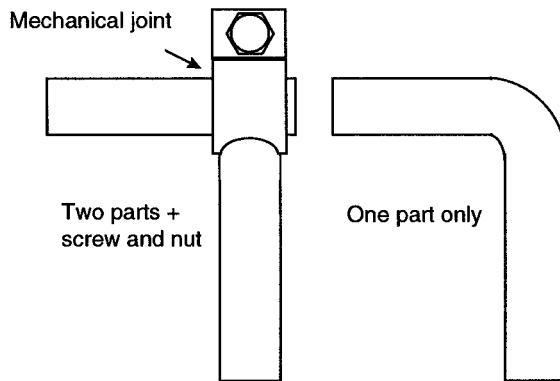
FIGURE 26.6 Integrate or combine parts.
