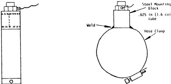
FIGURE 17.5 Hand-arm vibration tool measurements using an instrumentated automotive hose clamp. (Adapted from Wasserman, D. 1987. Human Aspects of Occupational Vibration , Elsevier Publishers, Amsterdam, The Netherlands.)
