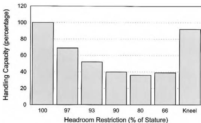
FIGURE 29.4 Handling capacity for stooping (percentages of full stature) and kneeling postures according to the IAP criterion. (From Ridd, J.E. 1985. Spatial restraints and intra-abdominal pressure. Ergonomics , 28(1): 149-166. With permission.)
