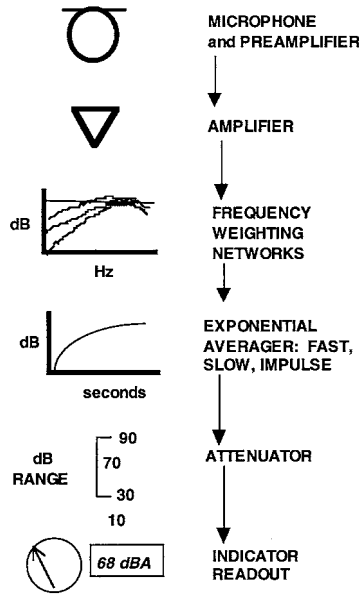
FIGURE 16.4 Block diagram of the basic functional components of a sound level meter.
