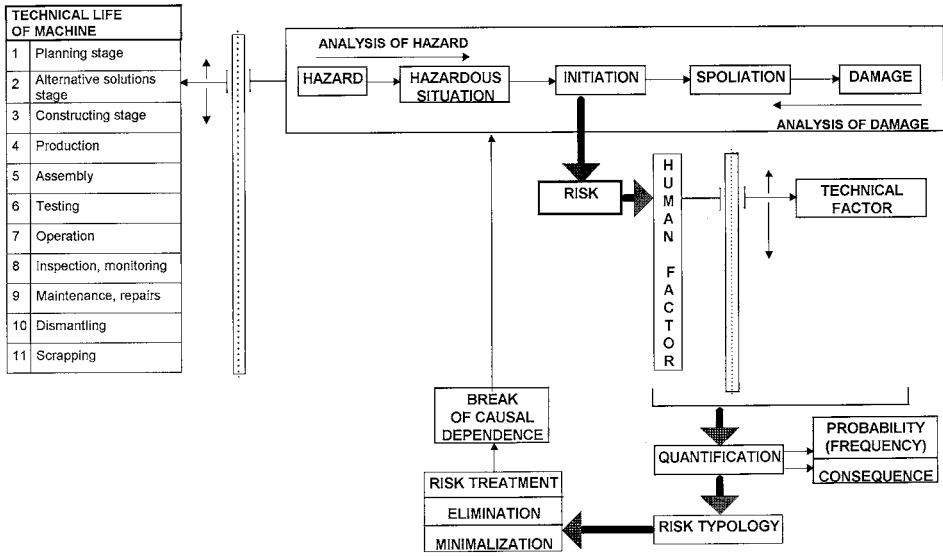
FIGURE 30.2 Scheme of analysis of technical systems risk.
