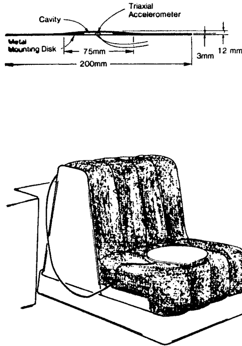
FIGURE 17.4 Whole-body vibration vehicle measurements using an instrumentated seat disc. (Adapted from Wasserman, D. 1987. Human Aspects of Occupational Vibration , Elsevier Publishers, Amsterdam, The Netherlands.)
