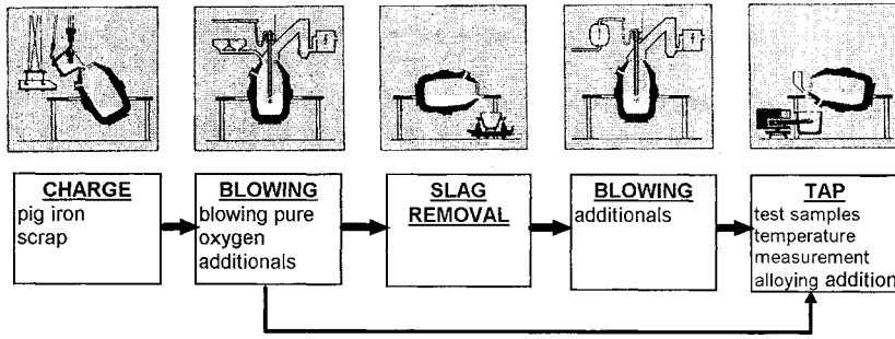
FIGURE 30.4 Scheme of blowing process.
