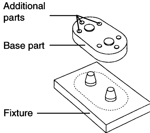
FIGURE 26.8 Provide a simple and reliable fixture for the base part. If possible, the base part should also serve as a fixture.
