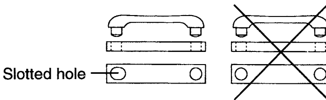
FIGURE 26.17 Reduce tolerances in part mating.
