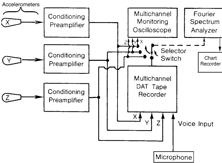
FIGURE 17.3 Basic triaxial vibration acceleration measuring system.
