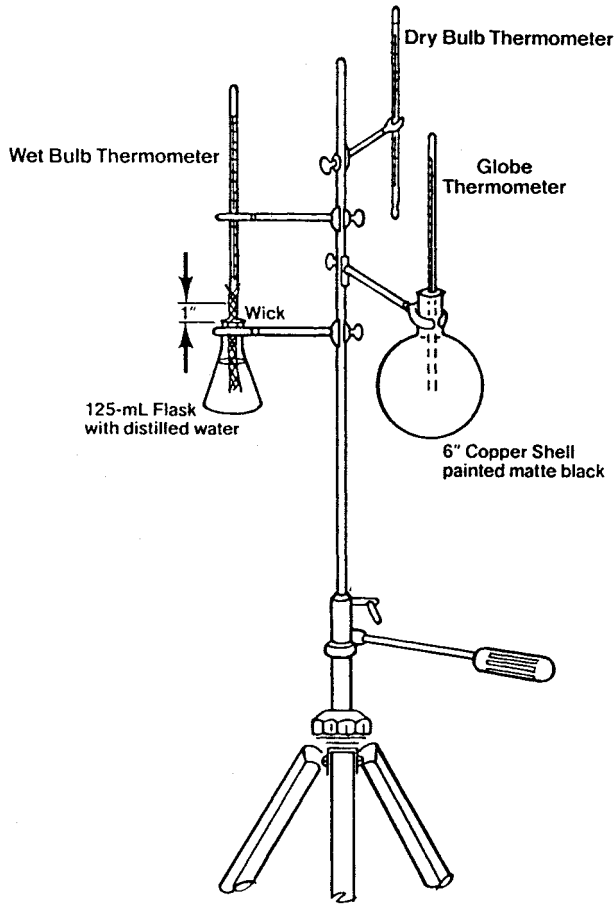
FIGURE 18.2 Instrument arrangement for outdoors WBGT measurements. (From Fundamentals of Industrial Hygiene , National Safety Council, 3rd edition, 1988, p. 269.)
