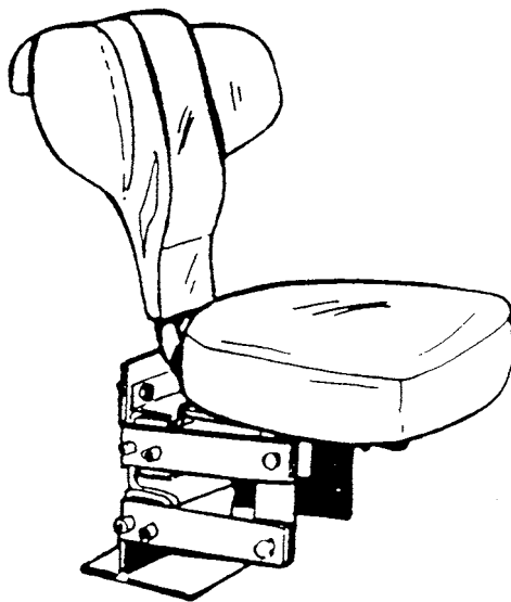
FIGURE 29.8 A prototype mining operator's seat developed using ergonomics principles and operator feedback. Note cutouts in the seatback, accommodating belt-worn personal protective equipment. (From McPhee, B. 1993. Ergonomics for the Control of Sprains and Strains in Mining . 36 pp., Handbook published by the National Occupational Health and Safety Commission (Worksafe Australia), Sydney. With permission.)
