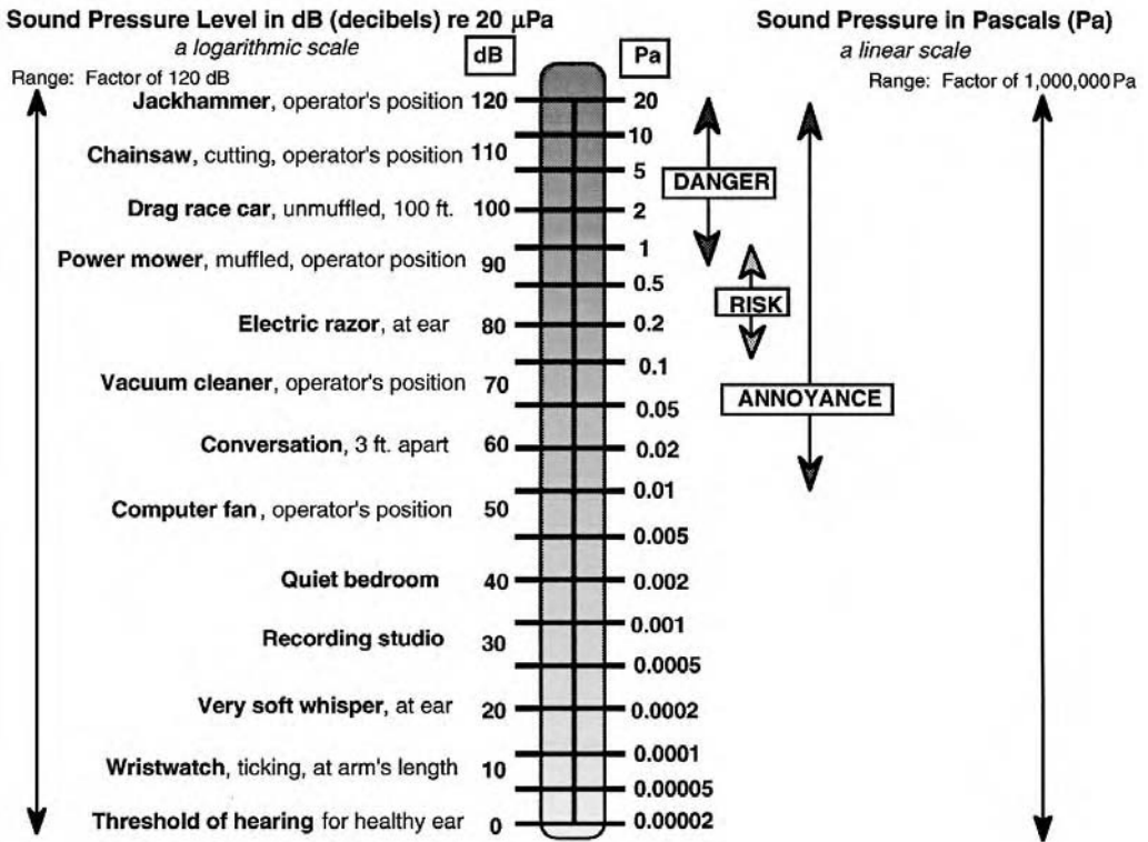
FIGURE 16.1 For typical sounds, sound pressure level values in dB and sound pressure values in Pascals.
