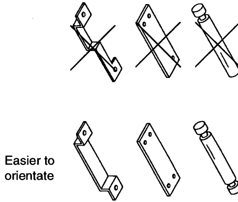
FIGURE 26.5 Use parts that are easy to orient, such as symmetrical parts.
