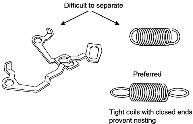
FIGURE 26.12 Avoid parts that nest or tangle.
