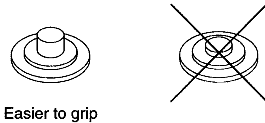
FIGURE 26.9 Improve parts handling by making parts easy to grip.
