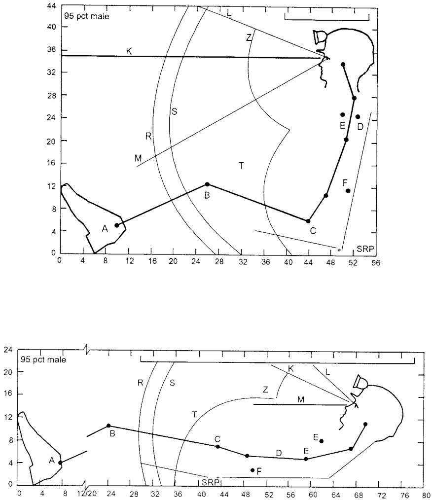
FIGURE 29.7 Seating space envelopes for 95th percentile miners in 107 cm (top) and 56 cm (bottom) cab heights. (From Canyon Research Group Inc. 1982. Human Factors Design Guidelines for Personnel Carriers , 37 pp., Canyon Research Group, Westlake Village, CA.)
