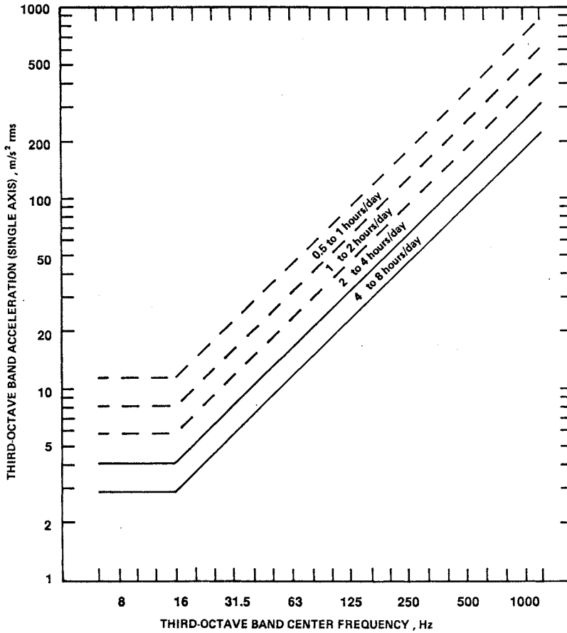
FIGURE 17.8 Hand-arm vibration curves for the separate evaluation of X,Y,Z axes rms accelerations (see text). (ANSI S3.34)
