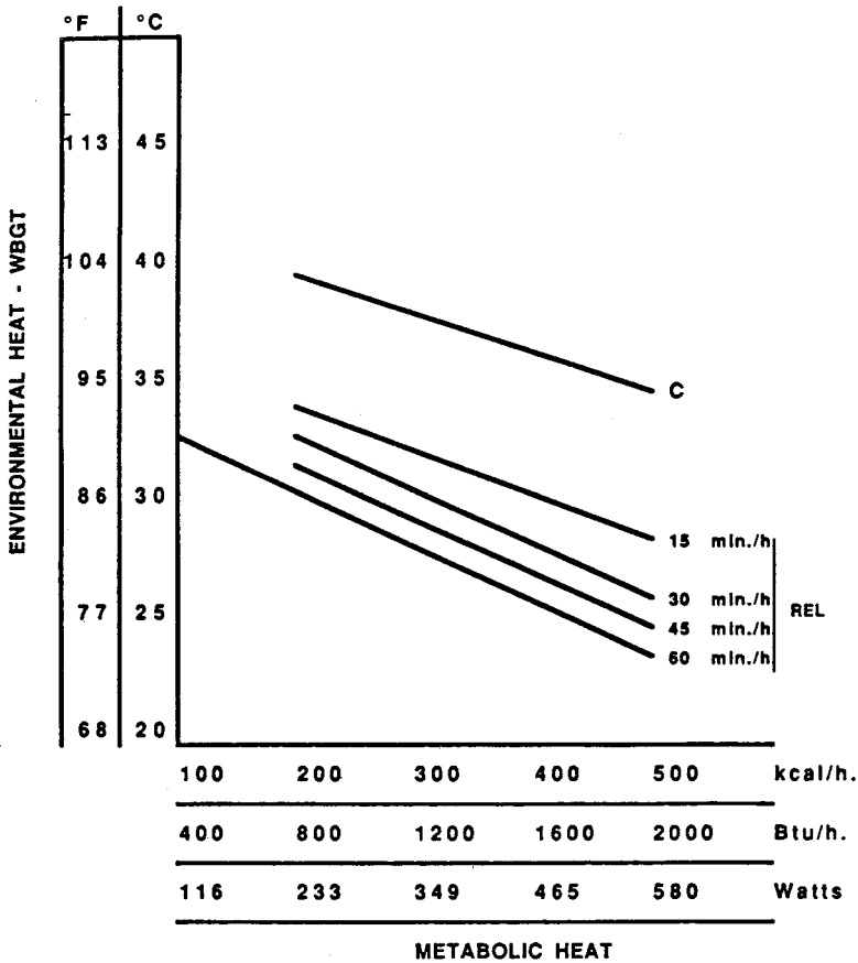
FIGURE 18.9 Revised heat stress limits (recommended exposure limits or REL) for acclimatized workers as a function of environmental heat (WBGT), intermitted work (min/h) and intensity of manual work as reflected by metabolic energy expenditure. The limits apply to a standard worker of 70 kg (154 lbs) body weight and 1.8 m 2 (19.4 ft 2 ) body surface. (From National Institute for Occupational Safety and Health [NIOSH] 1986, Criteria for a Recommended Standard: Occupational Exposure to Hot Environments revised criteria [NIOSH Publication No. 86-113].)
