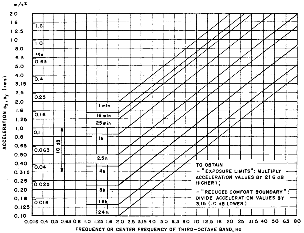
FIGURE 17.7 (FDP) Whole-body vibration curves separately used for X, Y axes rms acceleration evaluations. (ANSI S3.18, ISO 2631, EU)
