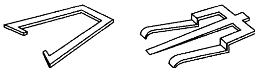
FIGURE 26.13 Avoid parts that are easily bent or parts that crack or chip.
