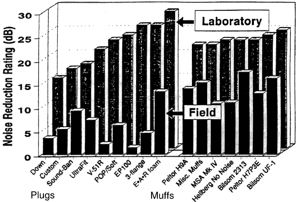
FIGURE 16.8 Comparison of hearing protection device NRRs by device type: manufacturers' laboratory data vs. real-world "field" data. (Adapted from Berger, E. H., Franks, J. R., and Lindgren, F. [1996]. International review of field studies of hearing protector attenuation, in A. Axelsson, H. Borchgrevink, R. P. Hamernik, P. Hellstrom, D. Henderson, and R. J. Salvi [Eds.], Scientific Basis of Noise-Induced Hearing Loss . [pp. 361-377], New York: Thieme Medical Publishers, Inc. With permission.)
