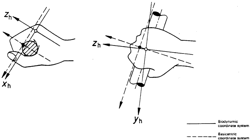
FIGURE 17.2 Hand-arm vibration measurements coordinate systems. (ANSI S3.34, ACGIH-TLV (HAV), EU, NIOSH #89-106)
