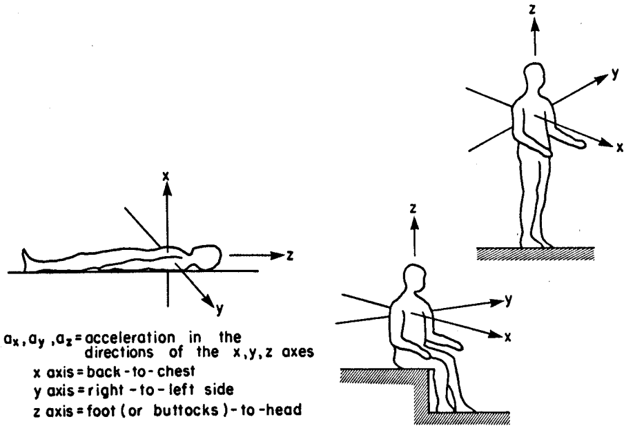
FIGURE 17.1 Whole-body vibration measurements coordinate system. (ANSI S3.18, ISO 2631, ACGIH-TLV (WBV), EU)
