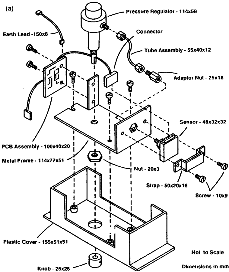
FIGURE 26.1a Example of product redesign for ease of assembly. The old design of the controller had 19 parts. The calculated assembly times are given in Table 26.1a. (From Boothroyd, G., Dewhurst, P. and Knight, W. 1994. Product Design for Manufacture and Assembly , Marcel Dekker, New York, NY. With permission.)
