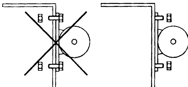
FIGURE 26.2 Avoid designs that lead to hidden assembly. From Willkrans, R. 1995. Design for Easy Assembly , IVF, publ. 95825, Gothenburg, Sweden. With permission.)
