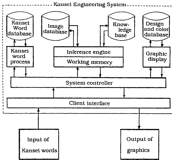
FIGURE 25.5 A system structure of the Kansei Engineering System.
