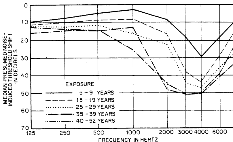
FIGURE 16.3 Cumulative auditory effects of years of noise exposure in a jute weaving industry. (Adapted from Taylor, W., Pearson, J., Mair, A. and Burns, W. [1964]. Study of noise and hearing in jute weavers. Journal of the Acoustical Society of America , 38, 113-120. With permission.)
