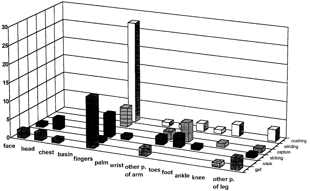
FIGURE 30.8 Injuries caused by mechanical parts of bridge crane.
