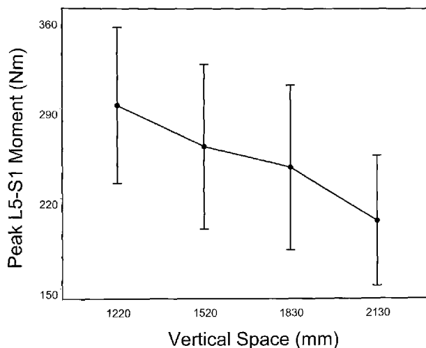
FIGURE 29.5 Relationship between vertical space restrictions and peak moment experienced during a cable hanging task. (From Gallagher, S., Hamrick, C.A., Cornelius, K., and Redfern, M. 1995. "Peak L5-S1 Moments Associated with a Cable Hanging Task," Poster Presentation at the 39th Annual Meeting of the Human Factors and Ergonomics Society Conference, San Diego, CA, October 9-13 1995.)
