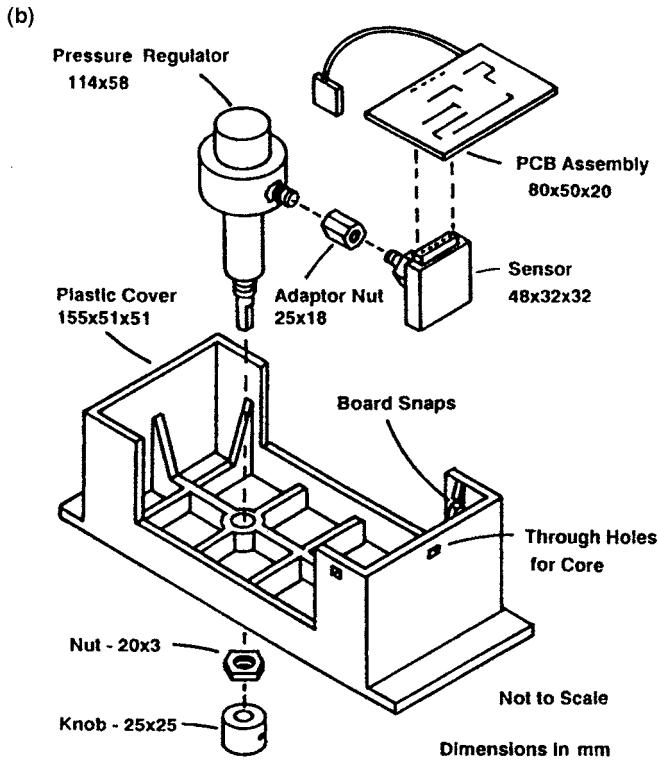
FIGURE 26.1b The new design of the controller had only 7 parts. The calculated assembly times are given in Table 26.1b. (From Boothroyd, G., Dewhurst, P. and Knight, W. 1994. Product Design for Manufacture and Assembly , Marcel Dekker, New York, NY. With permission.)
