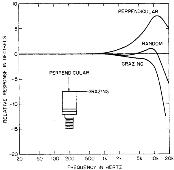
FIGURE 16.5 Frequency response of a hypothetical microphone for three angles of incidence. (Adapted from Peterson, A. P. G. [1979]. Noise measurements: Instruments, in C. M. Harris [Ed.] Handbook of Noise Control [pp. 5-1-5-19]. New York: McGraw-Hill. With permission.)
