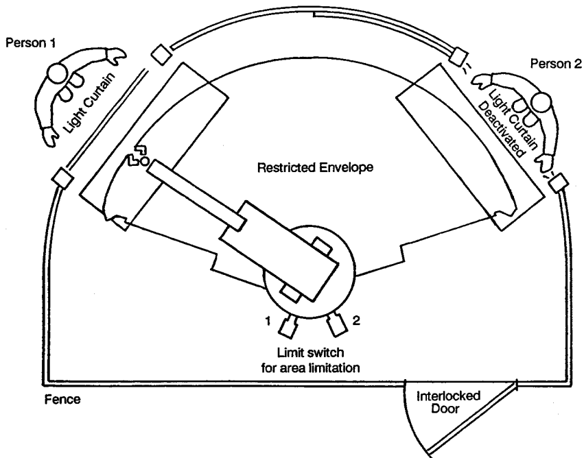
FIGURE 28.2 A schematic of a dynamic restricted human-robot cooperative workstation. The hazards for this cooperative workstation can be reduced by providing a robot controlled two-limit switch assembly. Each limit switch activates a light curtain where the robot arm is moving into for its routine task, while the other limit switch is deactivated allowing the second worker to perform the necessary tasks. (From American National Standard for Industrial Robots and Robot Systems — Safety Requirements . ANSI/RIA R15.06-1992, New York. With permission.)
