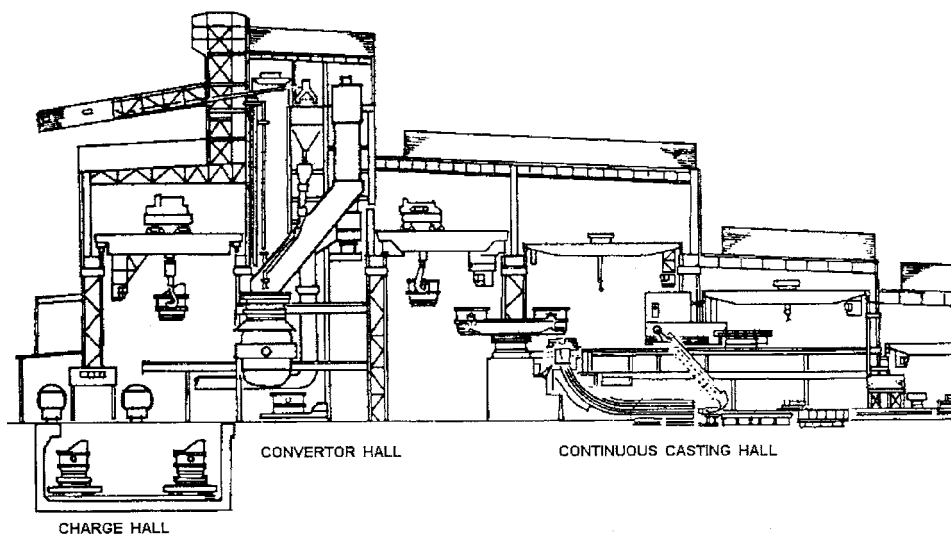
FIGURE 30.3 Converter steel plant scheme.
