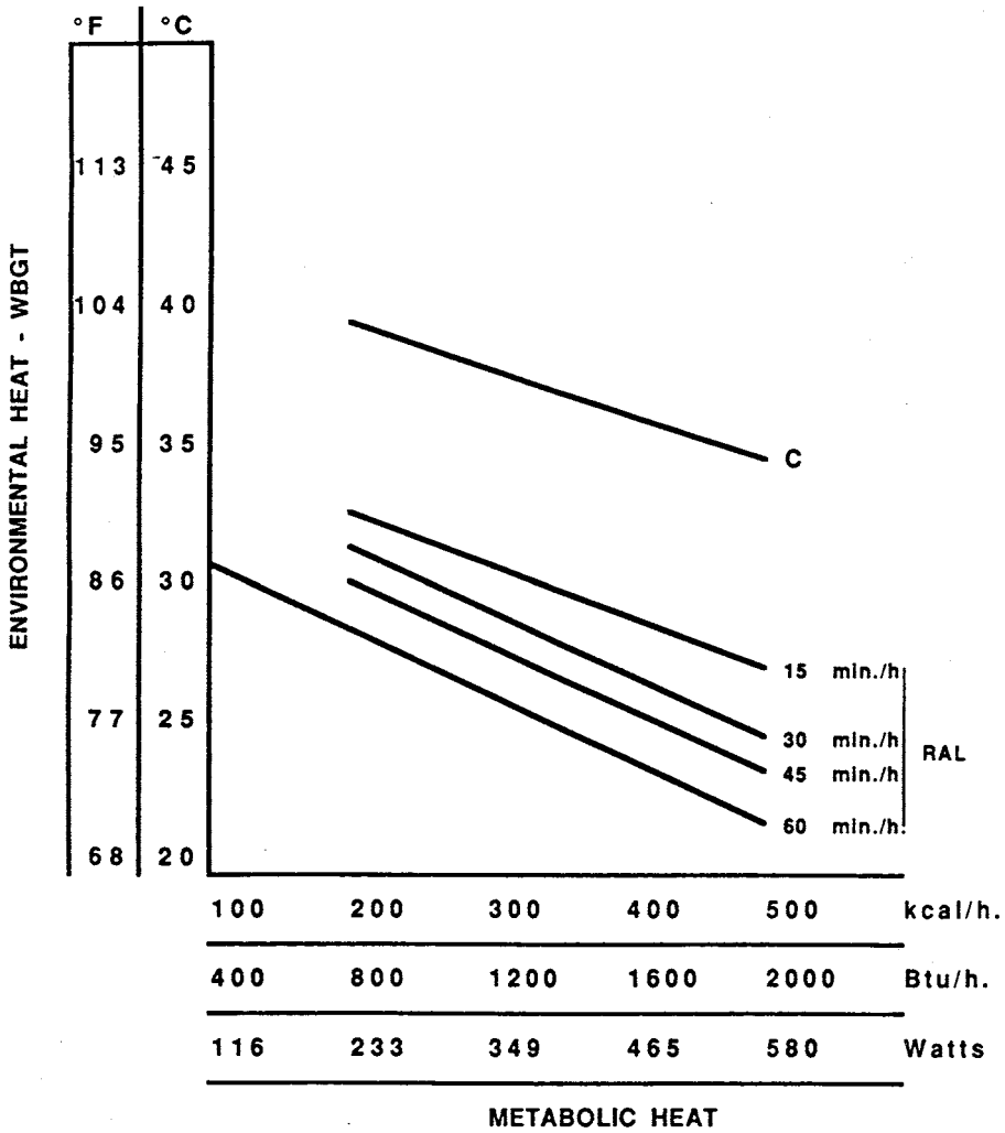
FIGURE 18.10 Revised heat stress limits (Recommended Alert Limits or RAL) for unacclimatized workers as a function of environmental heat (WBGT), intermitted work (min/h) and intensity of manual work as reflected by metabolic energy expenditure. The limits apply to a standard worker of 70 kg (154 lbs) body weight and 1.8 m 2 (19.4 ft 2 ) body surface. (From National Institute for Occupational Safety and Health [NIOSH] 1986, Criteria for a Recommended Standard: Occupational Exposure to Hot Environments revised criteria [NIOSH Publication No. 86-113].)
