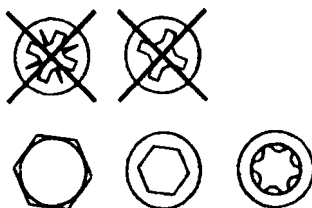
FIGURE 26.15 Use screws which do not create lifting forces on the tool. (From Willkrans, R. 1995. Design for Easy Assembly , IVF, publ. 95825, Gothenburg, Sweden. With permission.)
