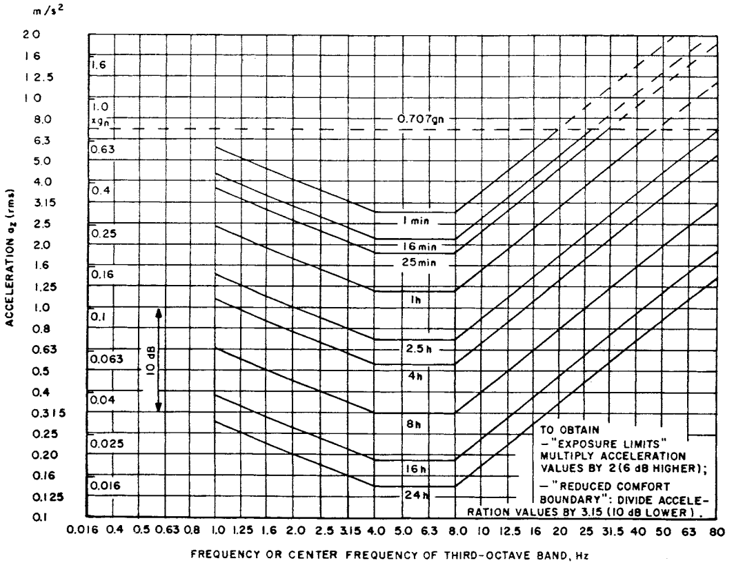
FIGURE 17.6 (FDP) Whole-body vibration curves for Z axis rms acceleration evaluation. (ANSI S3.18, ISO 2631, EU)
