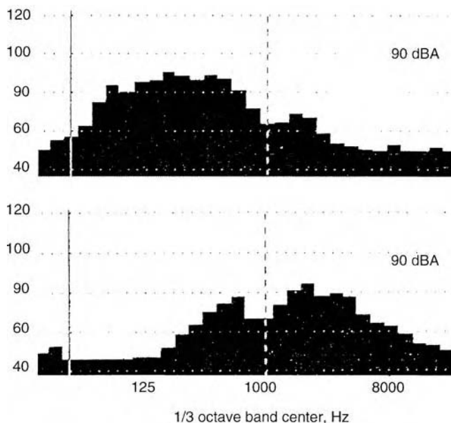
FIGURE 16.6 Spectral differences for two different noises which have the same dBA value.
