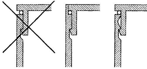
FIGURE 26.7 Integral fasteners and clips should be designed so that the operator can see, feel, or hear that the assembly has succeeded. (From Willkrans, R. 1995. Design for Easy Assembly , IVF, publ. 95825, Gothenburg, Sweden. With permission.)
