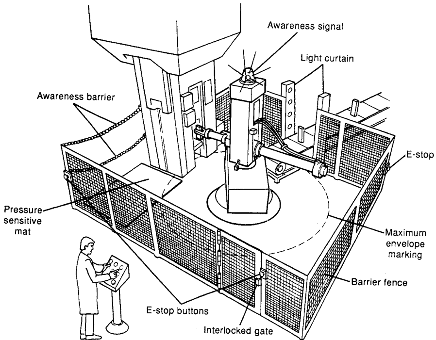
FIGURE 28.1 A schematic of a robotic workstation. This illustration includes a cylindrical robot, a conveyor belt feeding parts to the robot, an associated machine working on the workpiece, an operator with a computer control panel, and a typical array of safeguarding devices for worker protection in all zones of the workstation. (From American National Standard for Industrial Robots and Robot Systems — Safety Requirements . ANSI/RIA R15.06-1992, New York. With permission.)
