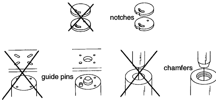
FIGURE 26.16 Facilitate assembly by using self-locating parts.
