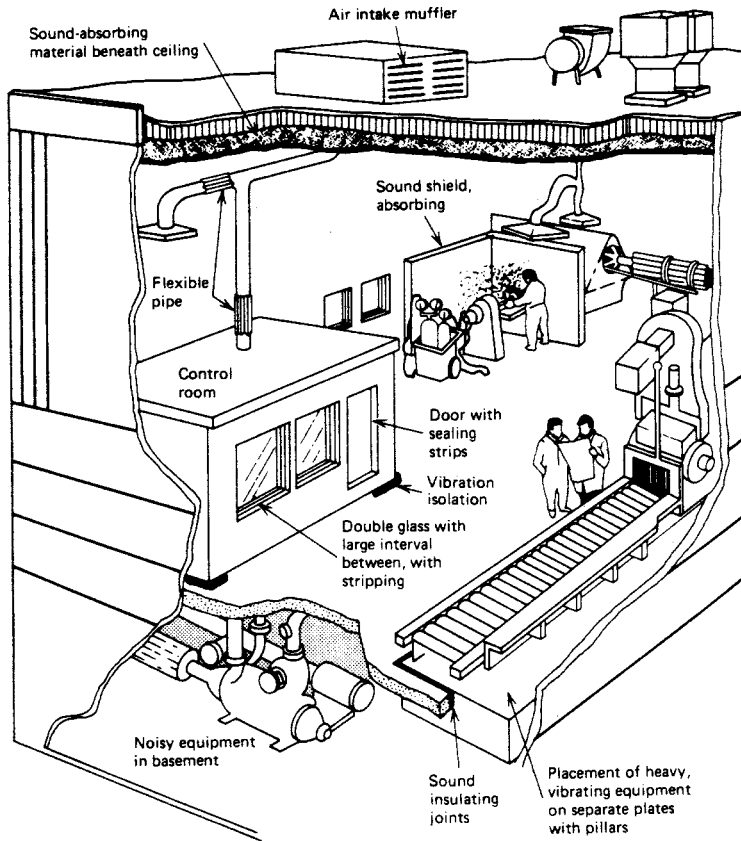
FIGURE 16.9 Examples of noise control implementation in an industrial plant. (Adapted from OSHA (1980). Noise Control, A Guide for Workers and Employers . Occupational Safety and Health Administration Report No. 3048. Washington, D.C., U.S. Department of Labor.)
