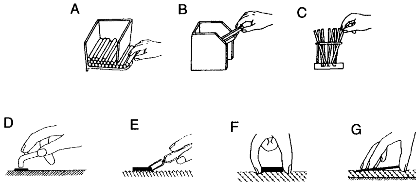
FIGURE 26.11 Gripping aids for an assembly workstation. (A) Self-feeding container. (B) Container with inclined opening. (C) A ring holder with smaller bottom diameter. (D) Use of vacuum gripper. (E) Tweezers or tongs used against a rippled table surface. (F and G) Gripping against a soft surface.
