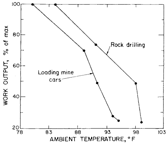
FIGURE 29.6 Effects of ambient temperature on miners' capacity to load mine cars and drill rock. (From Misaqi, F. L. 1984. Heat Stress in Mining . Safety Pamphlet No. 6, Mine Safety and Health Administration, Beckley, WV.)
