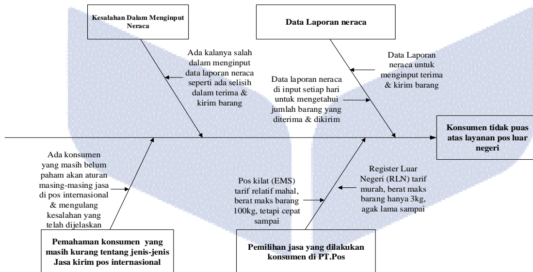
Gambar 1.1 Fishbone Diagram
