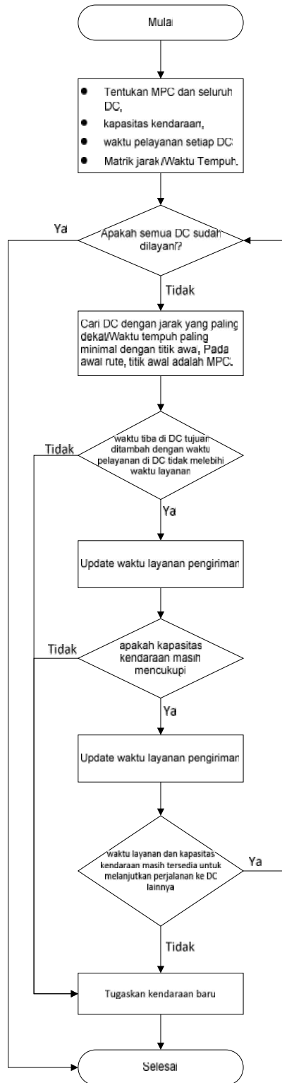
Gambar 4. FlowChart Algoritma Nearest Neighbor Heuristic
