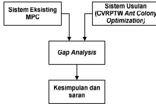
Gambar 5. Gap analysis
